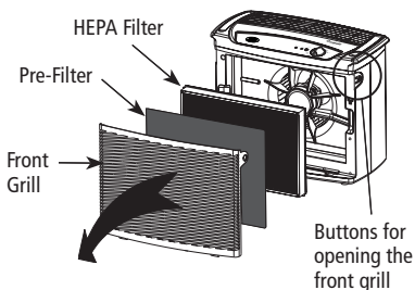
Figure 1 - Models 30117, 30119 & 30145
